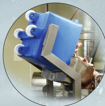
Easy To Use With Tipping Process
