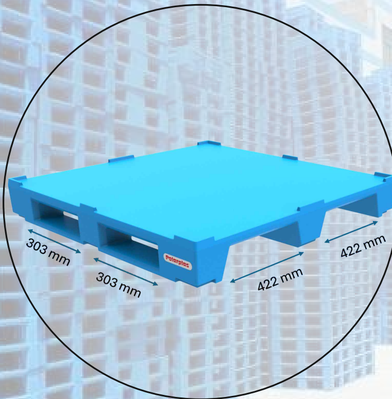
Stackable Design
